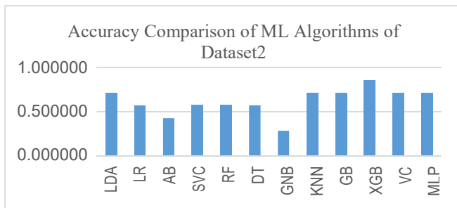
Fig. 2. Graph showing Comparison of classifiers (Dataset2)
